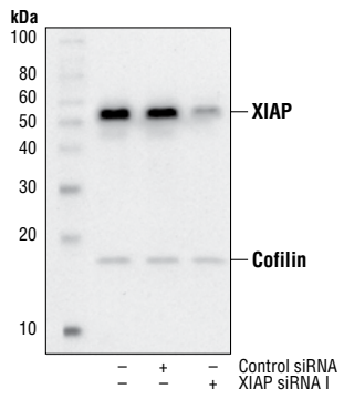
Western blot analysis of extracts from A549 cells, mock transfected or transfected with non-targeted (control) siRNA or SignalSilence® XIAP siRNA I, using XIAP Antibody #2042 and Cofilin Antibody #3312. The XIAP antibody confirms silencing of XIAP expression, while the cofilin antibody is used to control for protein loading and specificity of XIAP siRNA.
